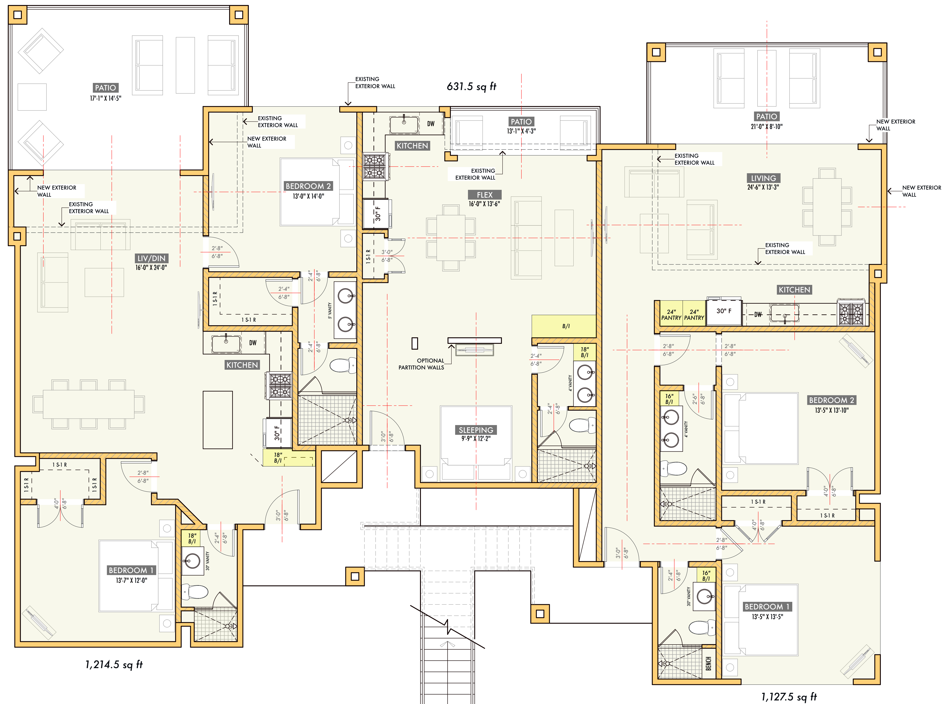
12 A1.1 First Level Plan 2 - 1 - 2 / Option B SCALE: 1/4" = 1'-0"
